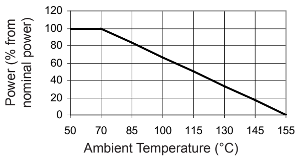
without Heatsink
